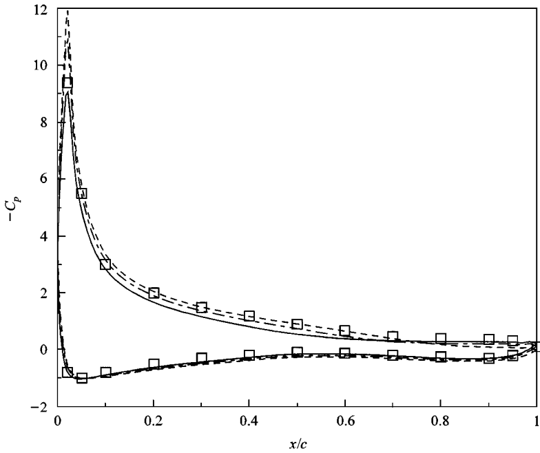
Figure 6. Comparison of the compute and measured pressure coefficient for \alpha = 17.6^\circ : ----, BL fully turbulent; —, BB fully turbulent; \square , experimental data by McCroskey et al. (1982); -.-.-, BB with transition.
